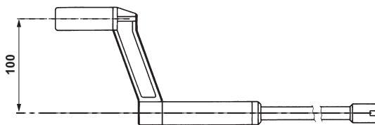
KLIKA S BAJONETEM / CRANK HANDLE WITH BAYONET
